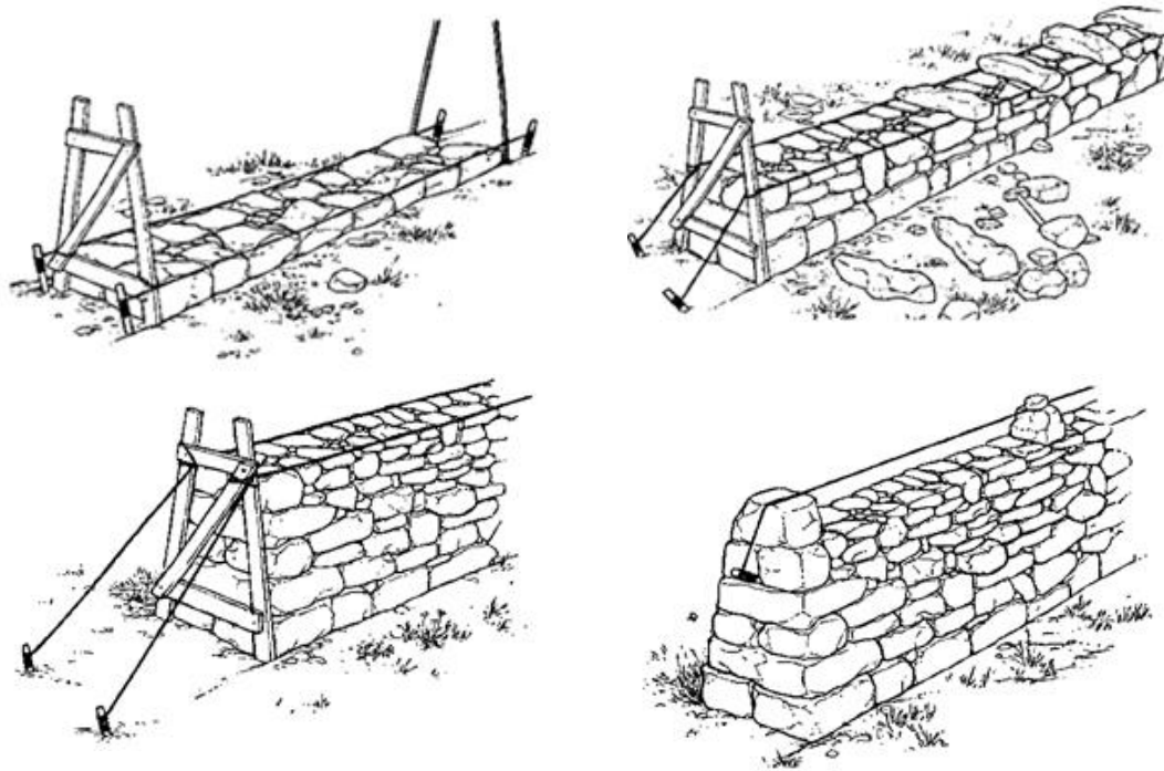
Construction phases of a rubble wall, from top left to bottom right: 1) Positioning of the first layer using larger-sized stones; 2) Positioning of the upper layers using smaller-sized stones and transverse stones; 3) Completion of the wall; 4) Closure and positioning of topping stones
